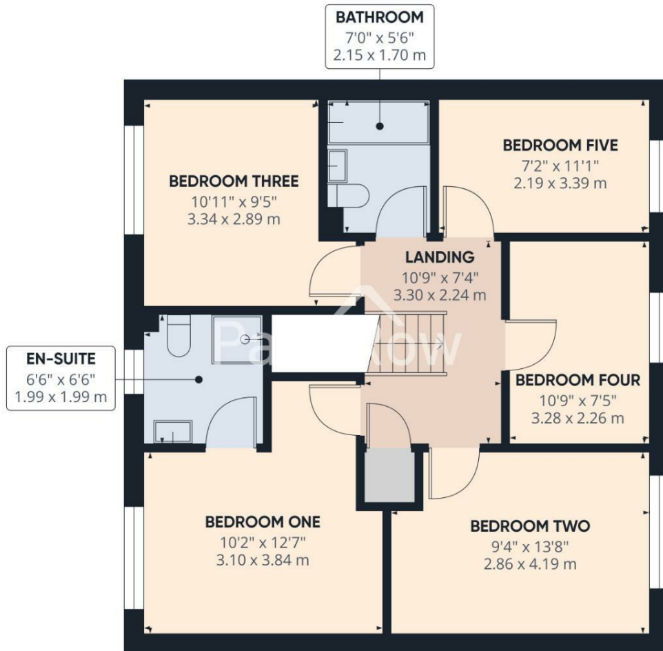
Floor 1 Building 1
